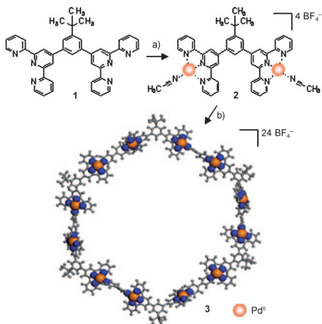
Scheme 1. Assembly of the palladium hexamer 3 represented by a computer-generated, partial space-filling model; reagents and conditions: a) MeCN, [\text{Pd}(\text{MeCN})_4](\text{BF}_4)_2 , 4 h, 25 °C; b) MeCN, 4,4'-bipyridine (1 equiv), 1 h, 25 °C. C gray, N blue, Pd II orange.
