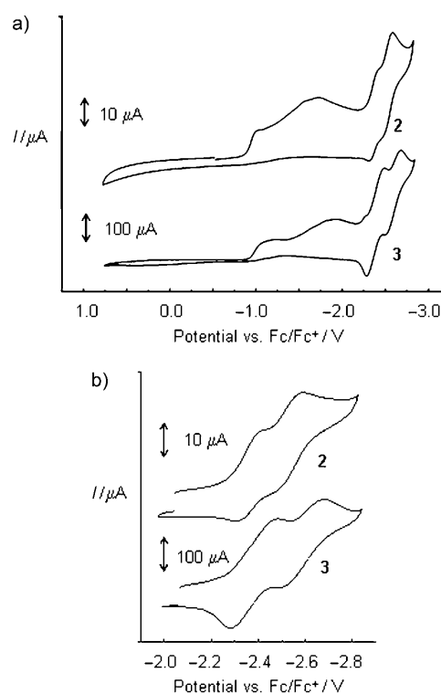
Figure 4. CV profiles of the bis Pd adduct 2 and hexamer 3 . The complete CV scans (a) and the expanded terpyridine-bipyridine regions (b) are depicted. \text{Fc}/\text{Fc}^+ = ferrocene/ferrocenium.
