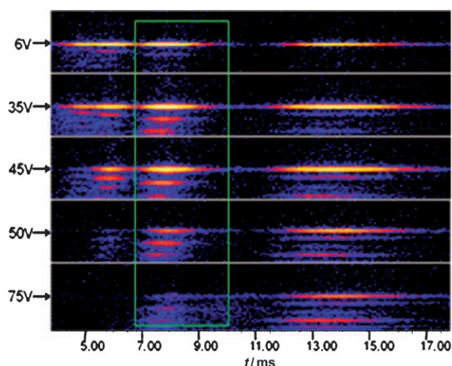
Figure 3. 2D ESI-TWIM-MS/MS plot of m/z 3174. The separated m/z 3174 components are indicated by arrows next to the trap cell voltages used for MS/MS. The signals for the [6L_1 + 12Pd + 6L_2]^{2+} macrocycles are surrounded by a green rectangle.
