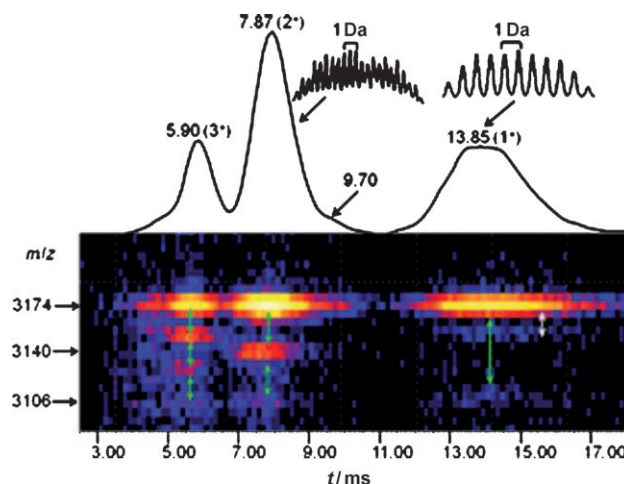
Figure 2. 2D ESI-TWIM-MS/MS plot for m/z 3174, acquired using a Waters Synapt quadrupole/time-of-flight (Q/TOF) mass spectrometer; m/z 3174 was mass-selected by Q for IM separation at a traveling wave height of 12 V and velocity of 350 \text{ m s}^{-1} ; trap and transfer voltages were set at 6 V and 40 V, respectively (see the Supporting Information for complete experimental details). After separation, m/z 3174 gives rise to signals at 5.90, 7.87, and 13.85 ms, corresponding to triply charged aggregates (5.90 ms), cyclic [6\text{L}_1 + 12\text{Pd} + 6\text{L}_2]^{2+} with 20 \text{F}^- and 2 \text{BF}_4^- counterions (7.87 ms) and linear species (13.85 ms). CAD with Ar, occurring in the transfer cell, causes losses of \text{BF}_3 and/or HF, which are indicated by green or white arrows respectively; m/z values of the fragments are marked on the y axis.
