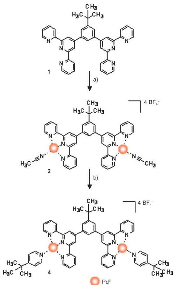
Scheme 2. Synthesis of the palladium model complex 4 ; reagents and conditions a) MeCN, [\text{Pd}(\text{MeCN})_4](\text{BF}_4)_2 , 4 h, 25 °C; b) MeCN, 4- tert -butylpyridine (2 equiv), 1 h, 25 °C. Orange spheres = \text{Pd}^{\text{II}} .
