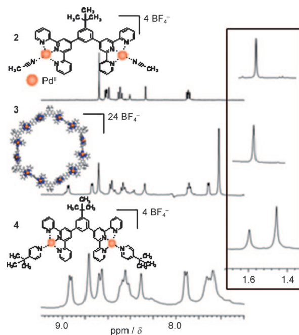
Figure 1. 1 H NMR spectrum ( \text{CD}_3\text{CN} ) of complexes 2 , 3 , and 4 showing the aromatic and tert -butyl regions. Orange spheres = Pd II .
